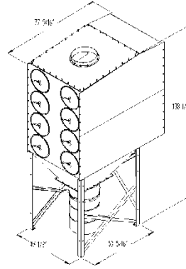
MPJC-H8D-B Drum & Hopper Configuration
